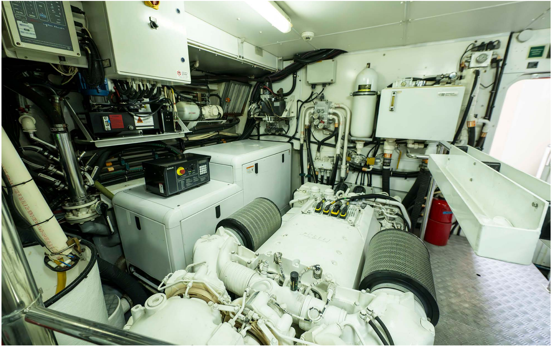
Engine room
