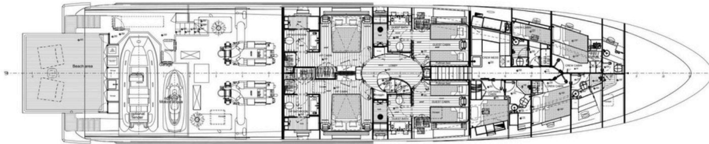
Lower deck
