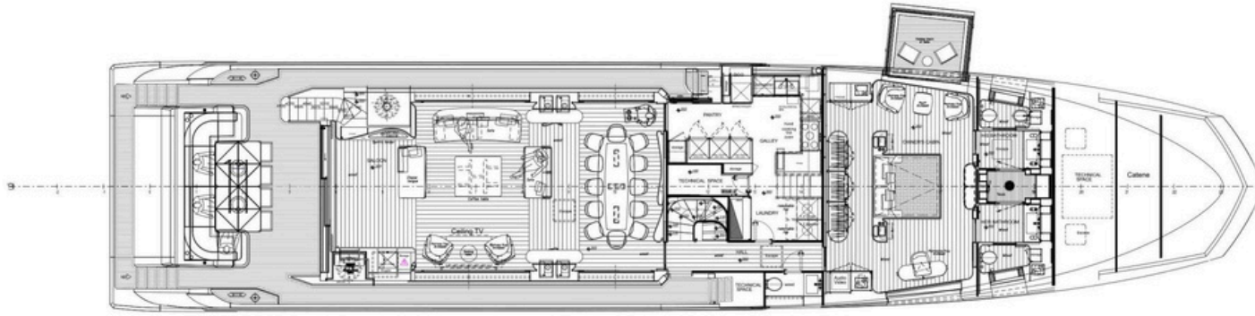
Main deck
